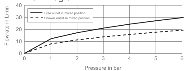
Flow Diagram
